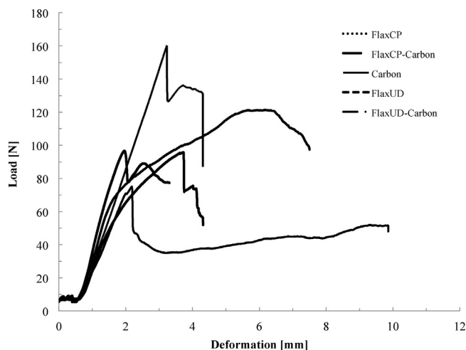
Fig. 3. Load deformation curves for different specimens.
