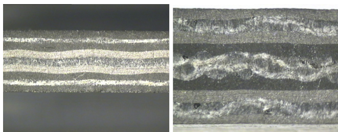
Fig. 7. Cross-sections of: (a) FlaxUD carbon and (b) FlaxCP carbon.
