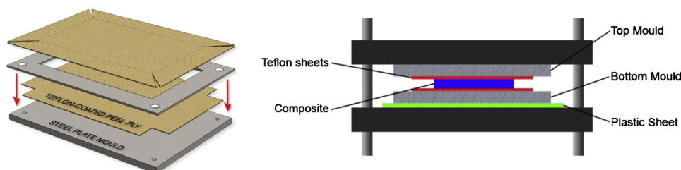
Fig. 1. Mould and compression moulding schematics.
