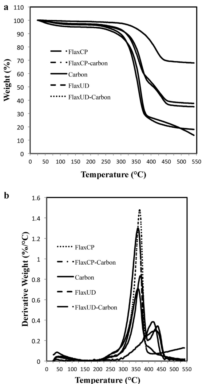
Fig. 8. (a) Thermogravimetric traces for different samples and (b) DTG traces for different samples.
