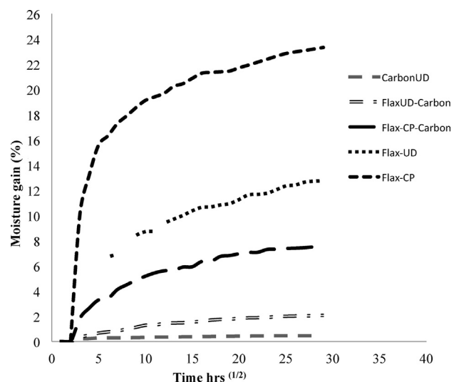
Fig. 2. Water absorption curves for flax and flax/carbon hybridised samples.
