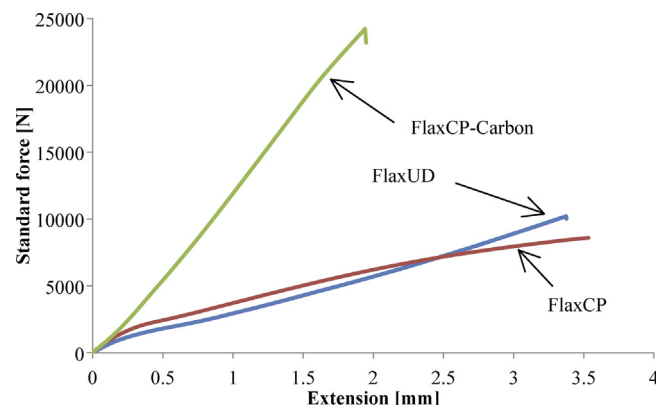
Fig. 5. Load extension curves for different samples in tensile testing.
